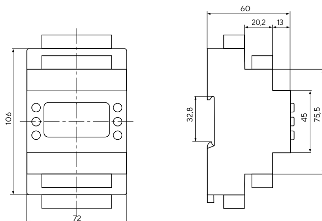
PLC-150-CPU-09U34U-0D, PLC-150-CPU-18U15U-1D
