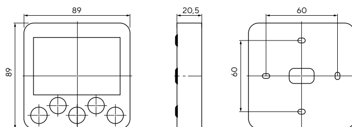
PLC-150-HMI-0000V1-0D
